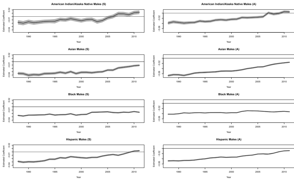
FIG. 1. Estimated racial wage gaps (coefficients of race indicators) for yearly males' regressions in synthetic data (left) and confidential, authentic data (right).
