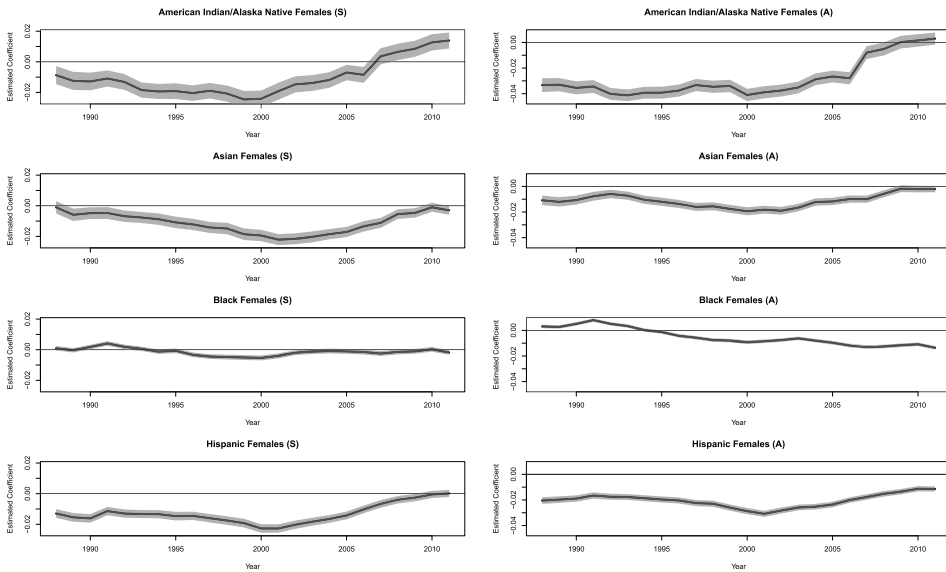
FIG. 2. Estimated racial wage gaps (coefficients of race indicators) for yearly females' regressions in synthetic data (left) and confidential, authentic data (right).
